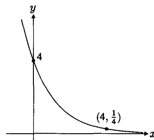
(c) a > 0, b > 0, b^2 = 4ac
